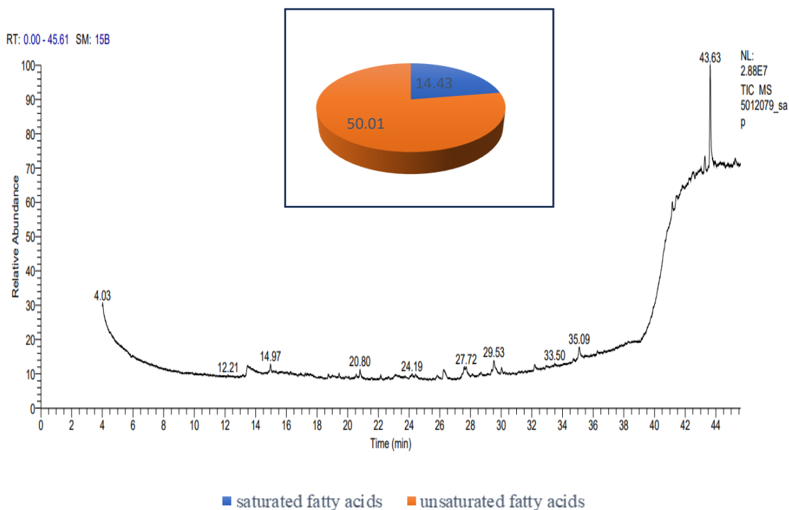
Figure 1. GC/MS chromatogram of the saponifiable matter of S.australe
