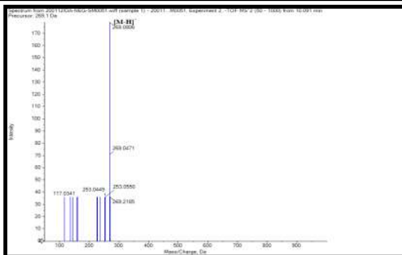
Apigenin
