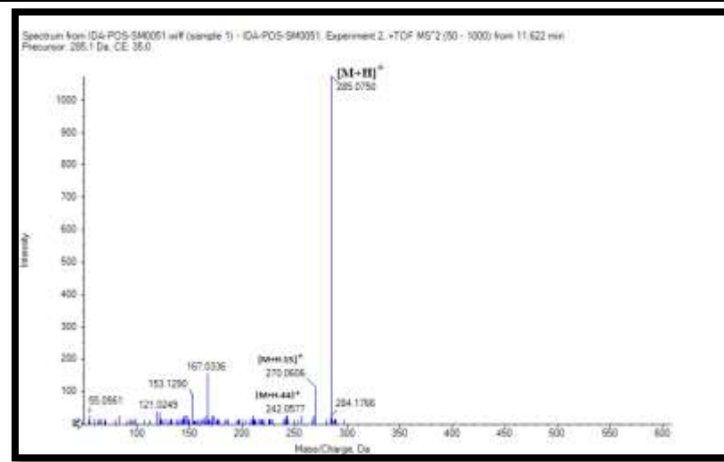
Acacetin
