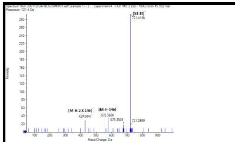
Dihydroxy spirostan-ene-deoxyhexoside
