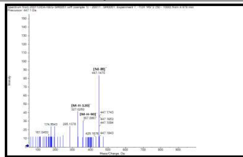
Luteolin-8-C-glucoside
