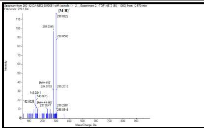
3,5,7-trihydroxy-4' methoxyflavon
