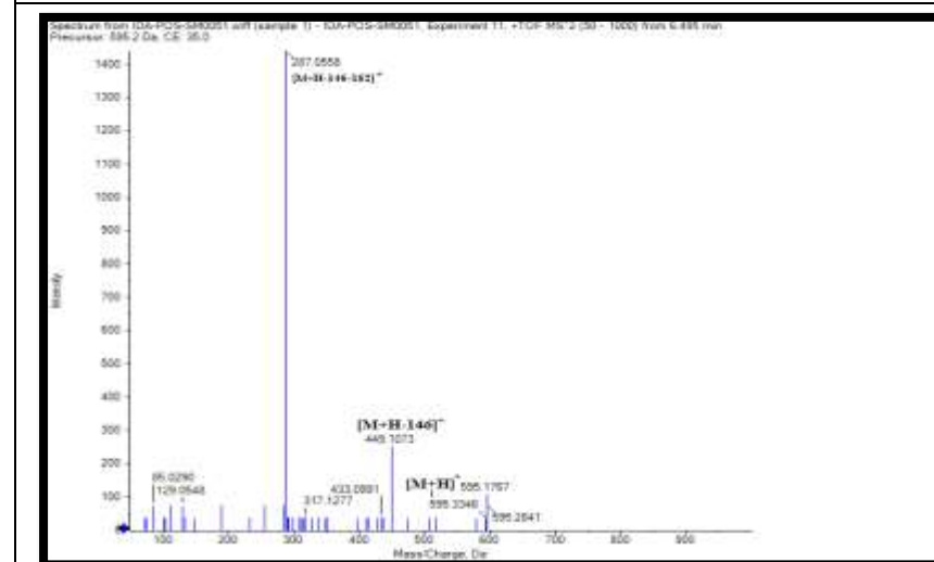
Kaempferol-O-neohesperidoside
